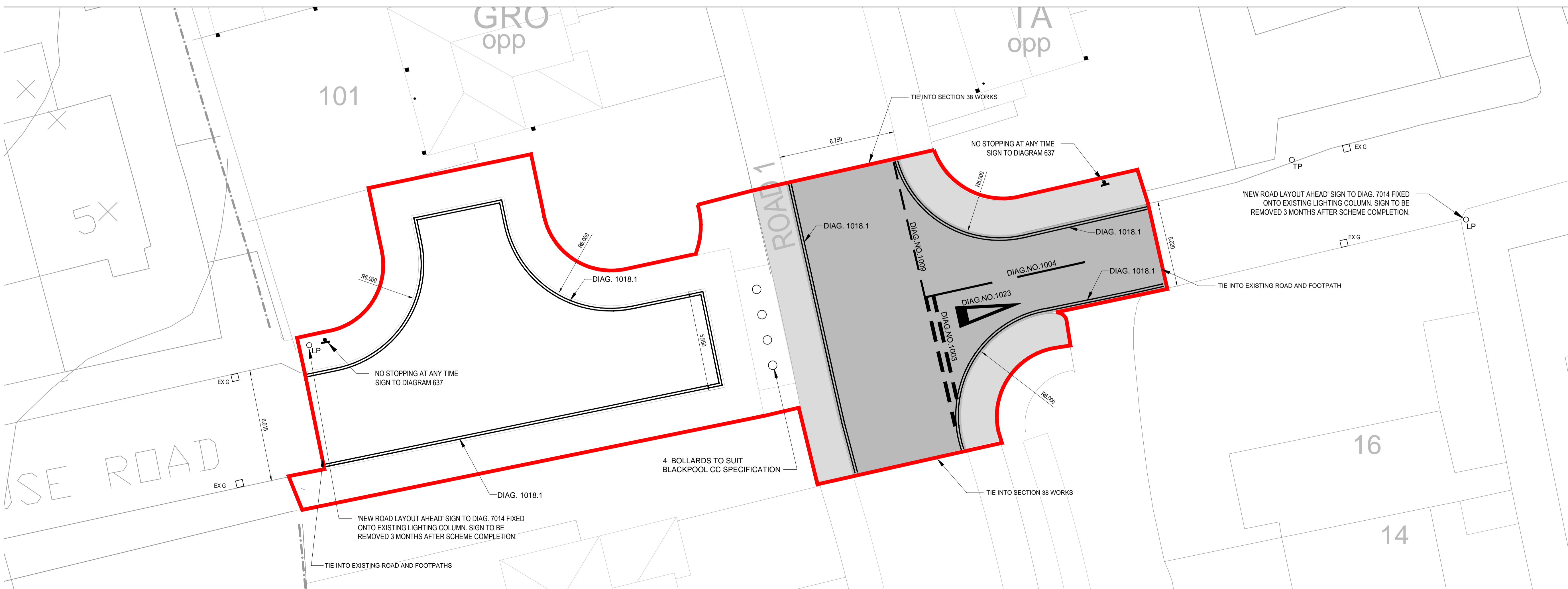
JUNCTION SCALE 1:150
